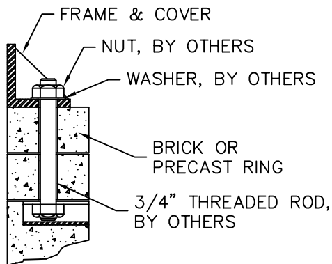
CONNECTION DETAIL
