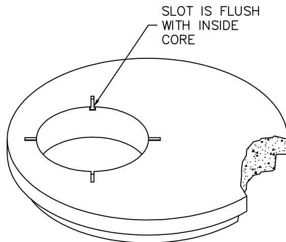
STANDARD FLAT SLAB SECTION
