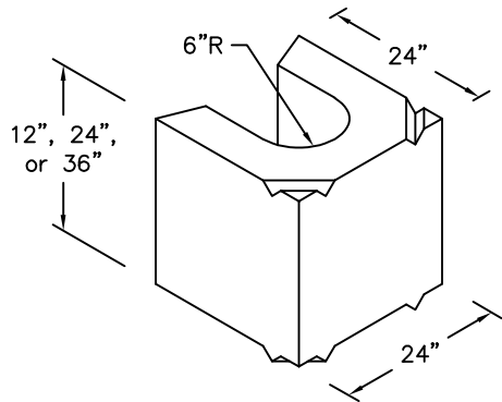
COLLAR DETAIL
